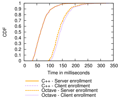
Figure 1: CPU time for enrollment
