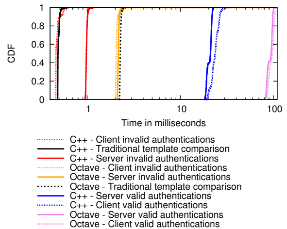
Figure 2: CPU time for authentication
